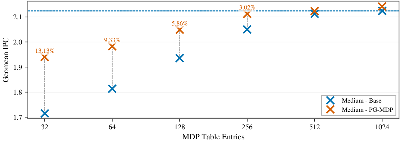
Fig. 5: Base and improved IPC across SPECspeed 2017 for increasing XS Store Set [26] sizes on a medium core (ROB=256). IPC gains increase over the small core, but for the baseline MDP size (256 entries), IPC improvement is still 0.5% smaller.
