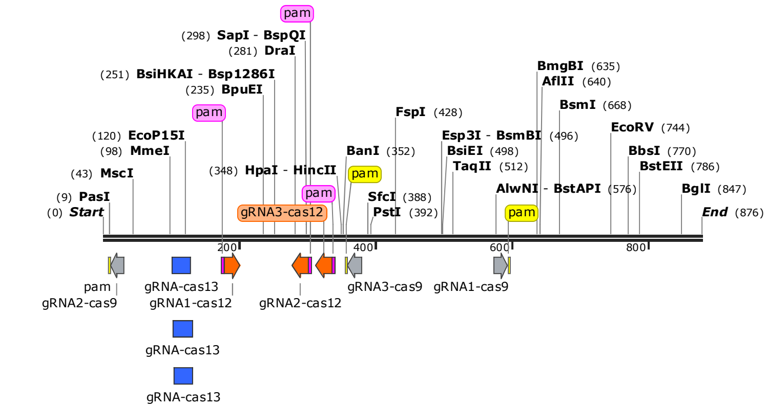
snappgene_blaCTX_viewer 876 bp
