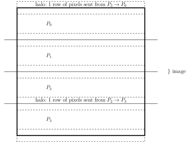
Fig. 1: Distribution of data between processes
