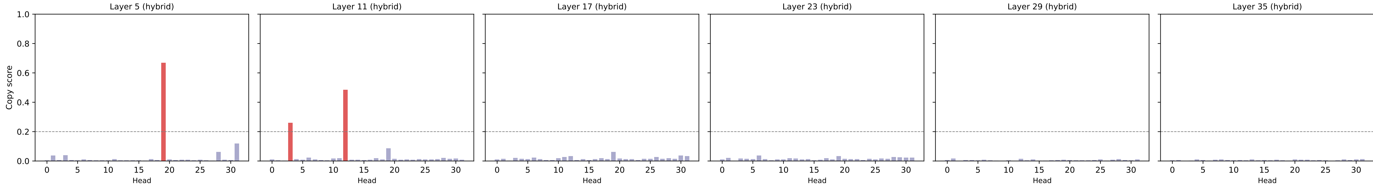
Copy score per attention head — Zamba2-1.2B hybrid layers (Red = high-copy head, likely induction-like)
