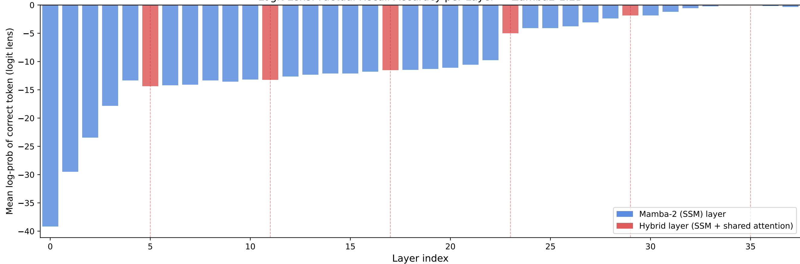
Logit Lens: Factual Recall Accuracy per Layer — Zamba2-1.2B
