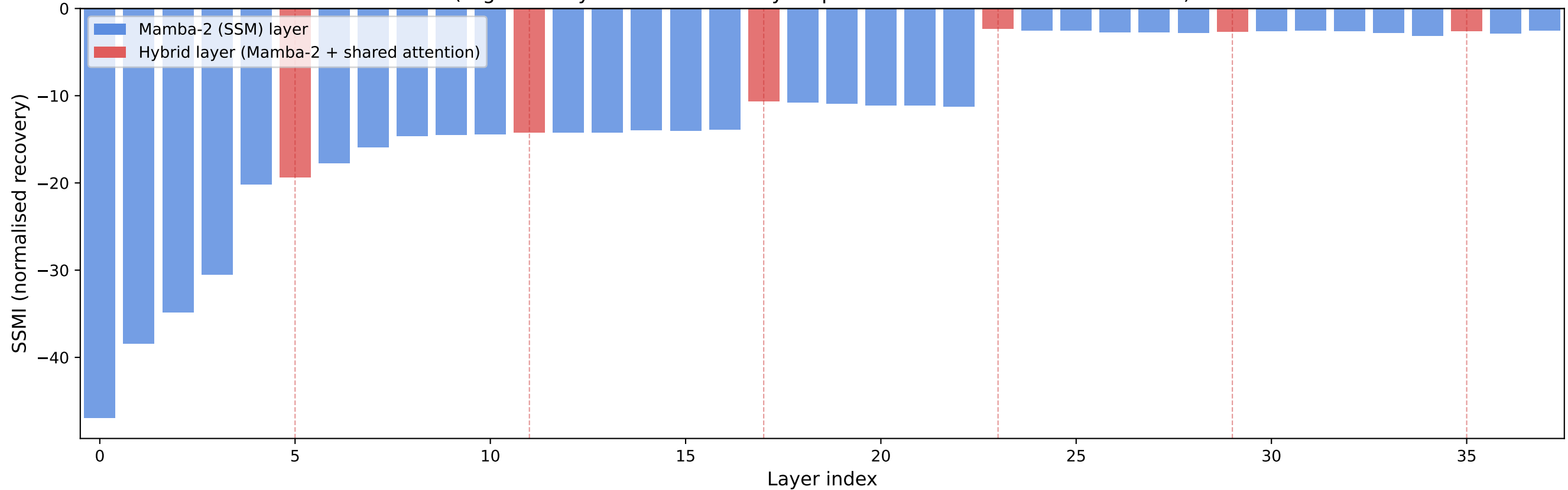
SSM Induction Score per layer — Zamba2-1.2B (Higher = layer is more causally responsible for induction-like behavior)
