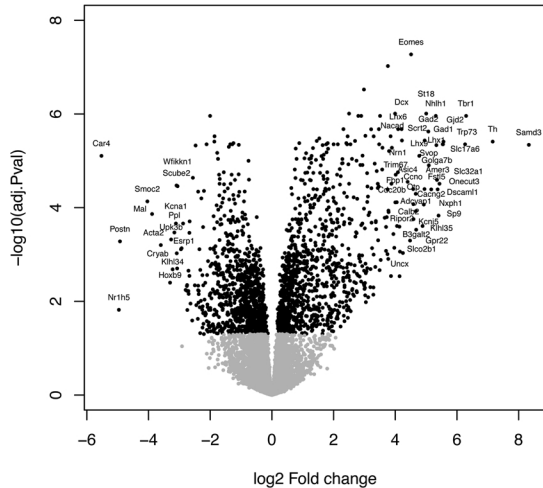
Mouse
