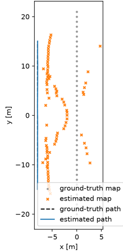
Fig. 4. Realistic 60 GHz map (joint MUSIC). Despite 8.5 cm range resolution, the estimated reflectors (orange) form a consistent phantom arc along the vehicle trajectory (LOS/floor paths), not the wall (grey, at x=0 ).
