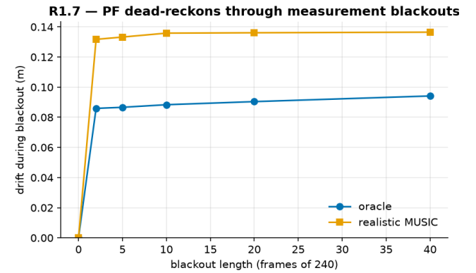
FIGURE 7. Blockage robustness. The particle filter dead-reckons through a total measurement blackout: a 40-frame (17% of run) outage adds \approx 0.1 m drift and re-locks immediately.
