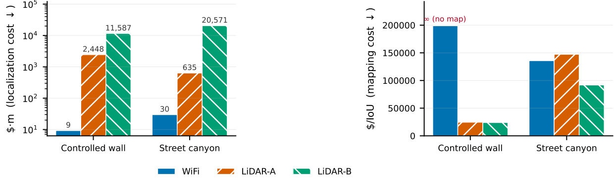
Fig. 3. Cost read together with accuracy. Left: localization cost (price \times ATE) — WiFi is one to two orders of magnitude better per dollar. Right: mapping cost (price per unit IoU) — WiFi buys no map coverage at any price.
