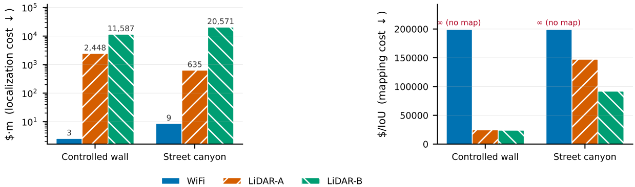
Fig. 4. Cost read together with accuracy. Left: localization cost (price × ATE) — WiFi is two to three orders of magnitude better. Right: mapping cost (price / IoU) — WiFi’s is infinite, because it buys no coverage at any price. LiDAR is priced at the tier we simulate.
