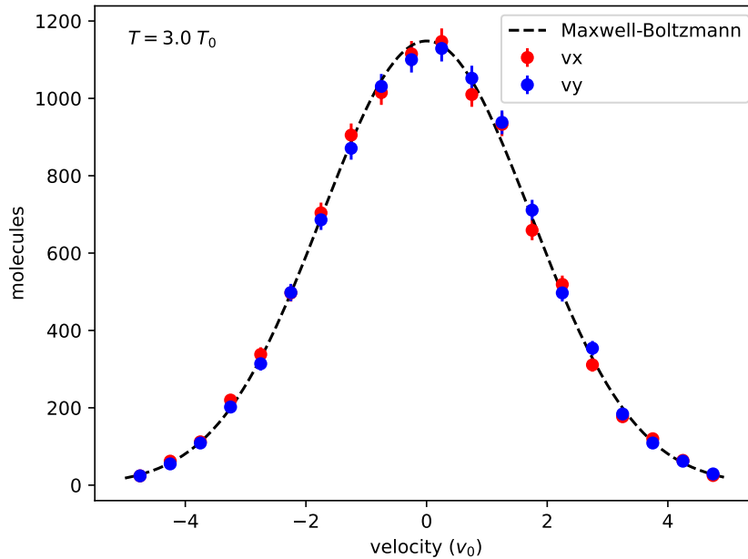
Figure 5: Thermal equilibrium.
