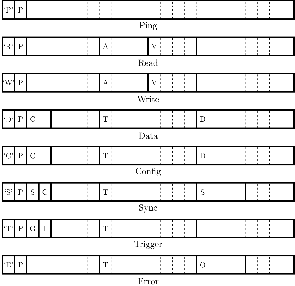
Figure 9: Layout of PACMAN message words by word type, showing field locations and sizes, labeled by the single character symbol from Table 12. The space between each pair of lines represents one byte, and each word is 24 bytes wide (192-bits). The least significant bit is to the left, the the least significant byte is a character field used to indicate the word type.
