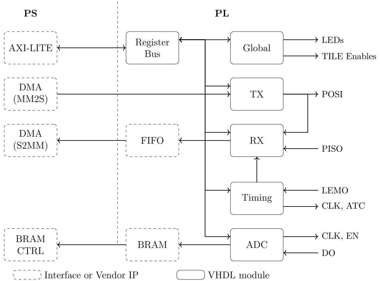
Figure 1: Top-Level Block Diagram of HW Demonstration Firmware
