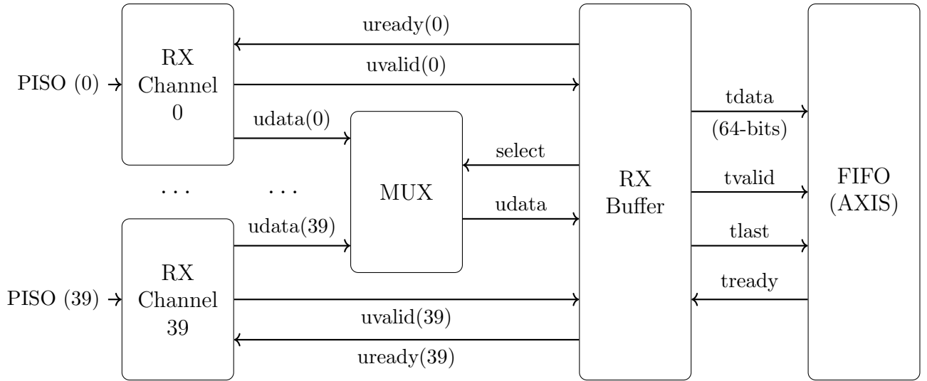
Figure 7: Data path in the RX Unit. Timestamps from each channels are MUXed in a similar fashion for inclusion in the stream. A secondary output of the MUX is used to provide a look register.
