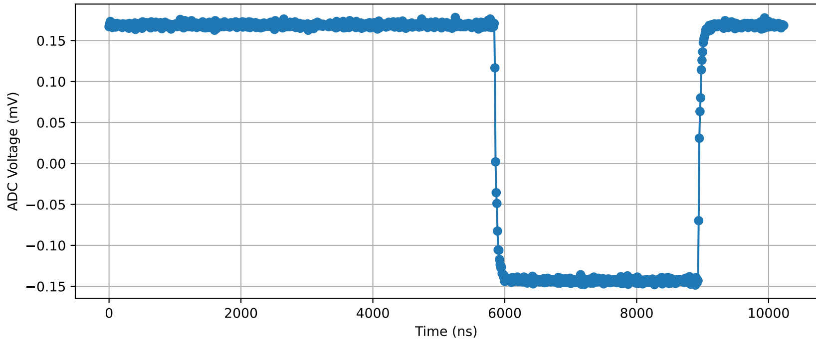
Buffer 0 (CONFIG=0x10000033, INPUT=0x0)
