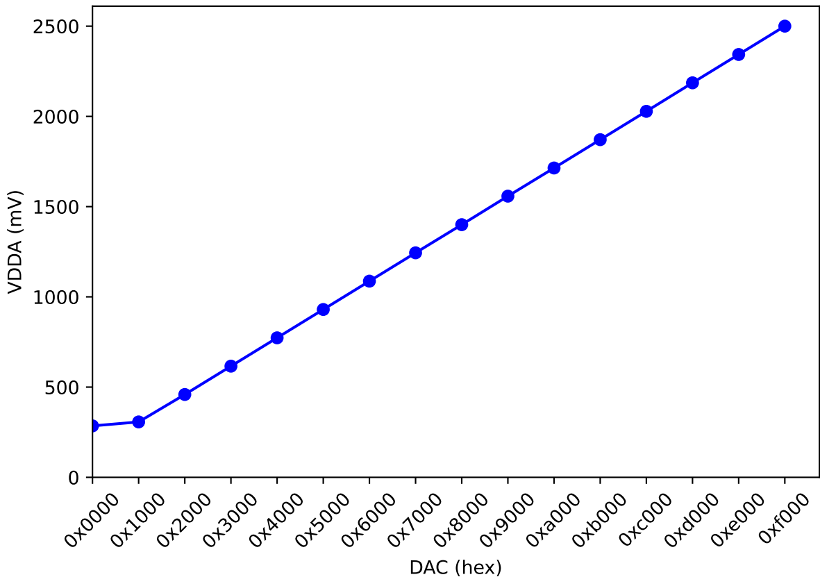
VDDA vs DAC
