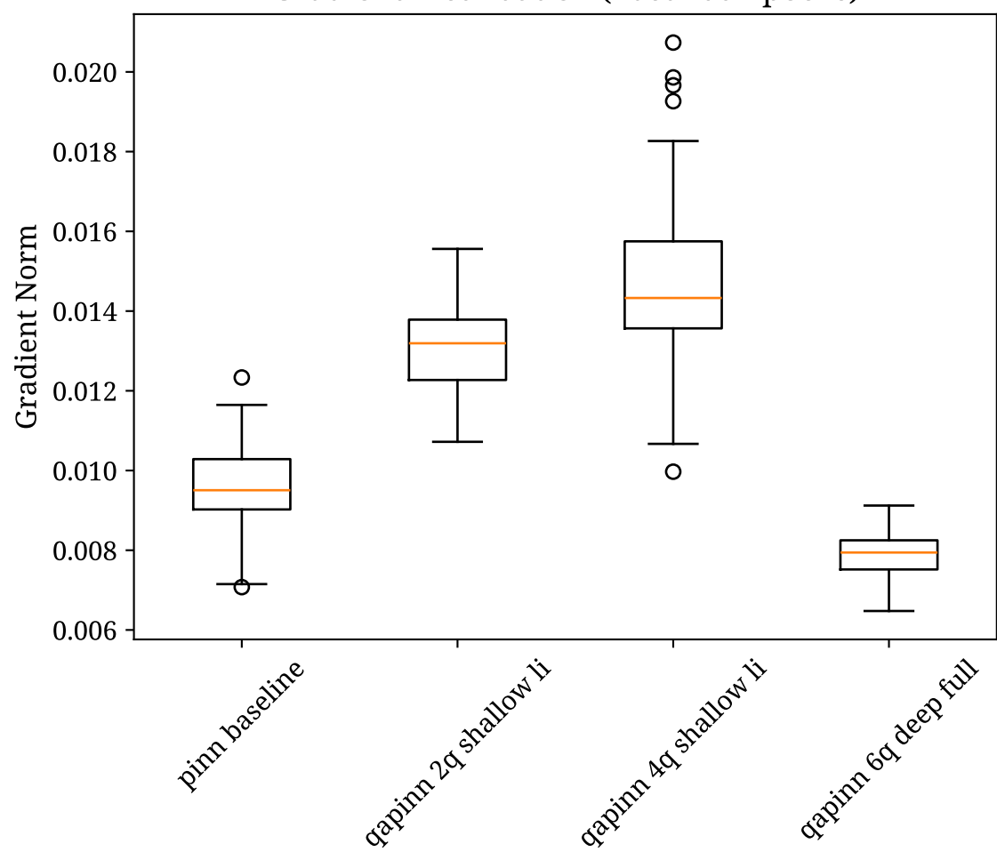
Gradient Scaling with Qubit Count
