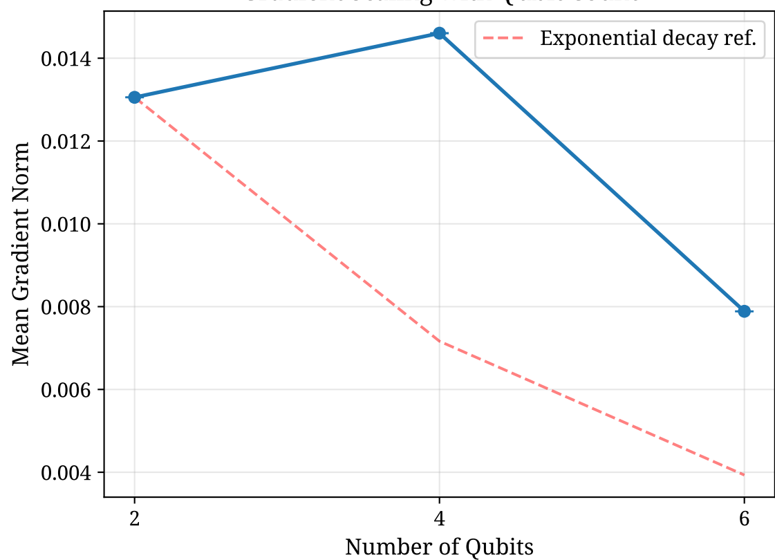
Gradient Scaling with Qubit Count
