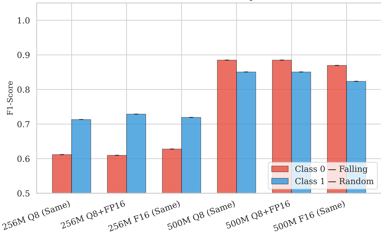
Class-wise F1-Score Comparison
