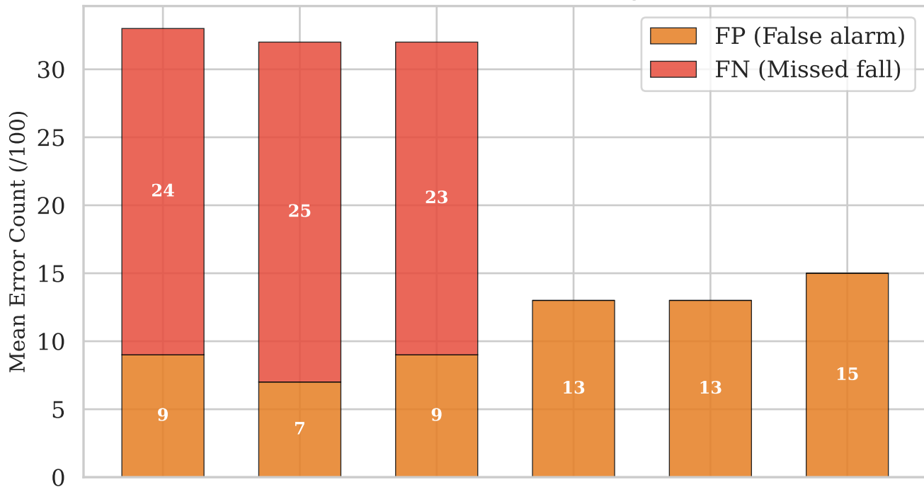
False Positive vs False Negative
