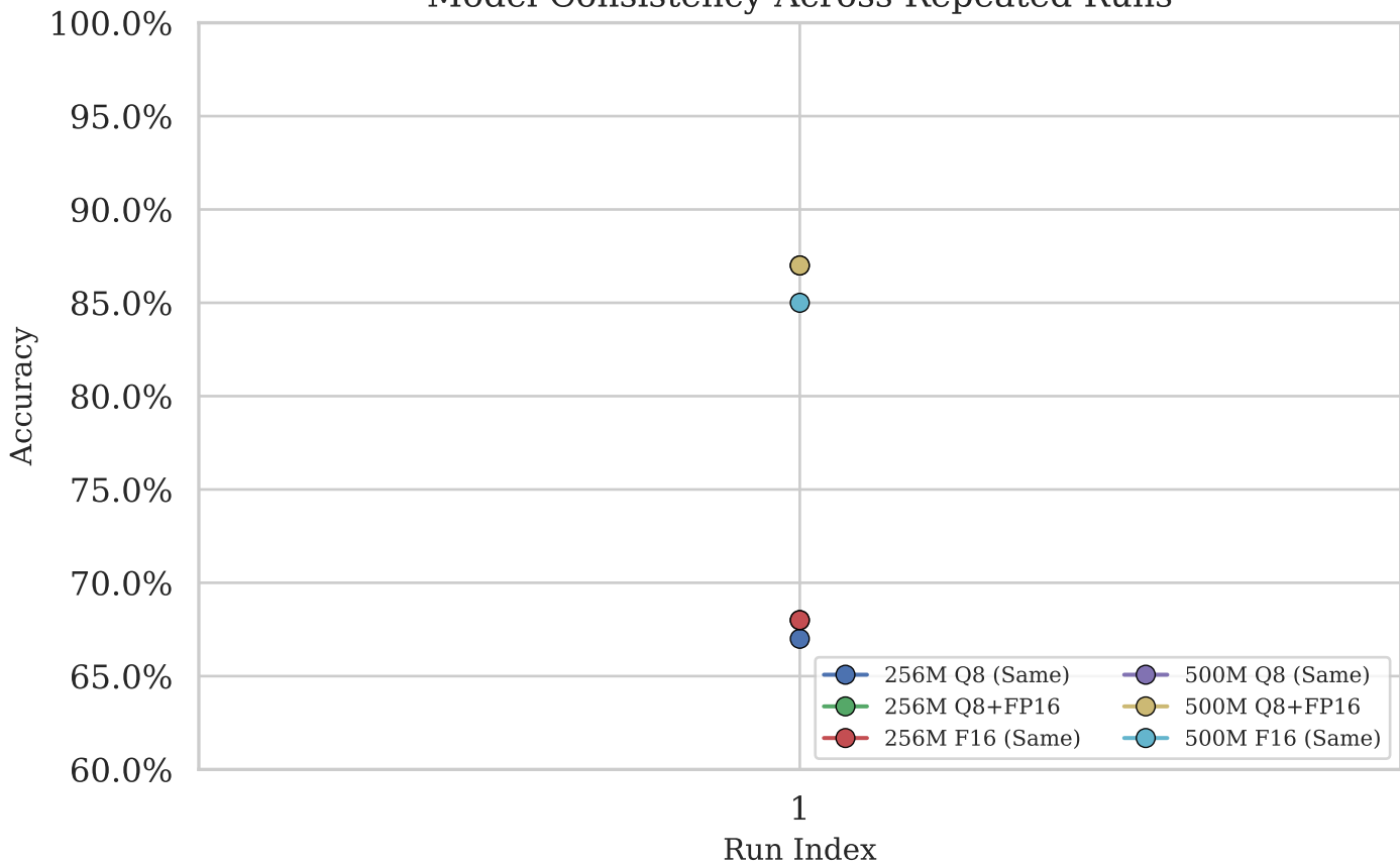
Model Consistency Across Repeated Runs
