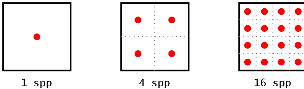
Figure 4.8: Multi-Sampling Grid
