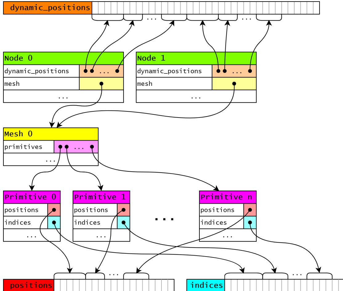
Figure 4.8: Usage of sub-buffers in a scene
