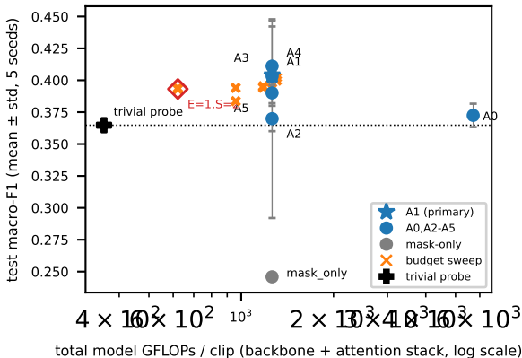
Accuracy vs. compute (detection cost excluded -- see text)
