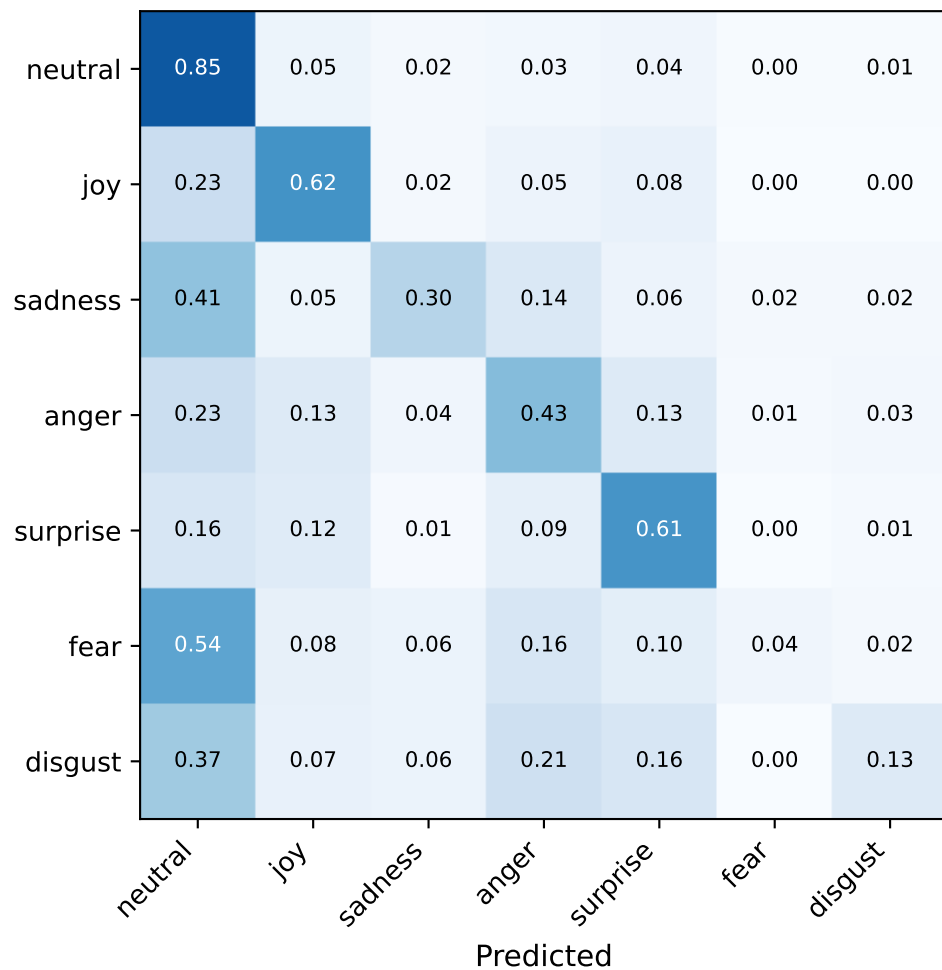
MELD (Full stack, seed 42)
