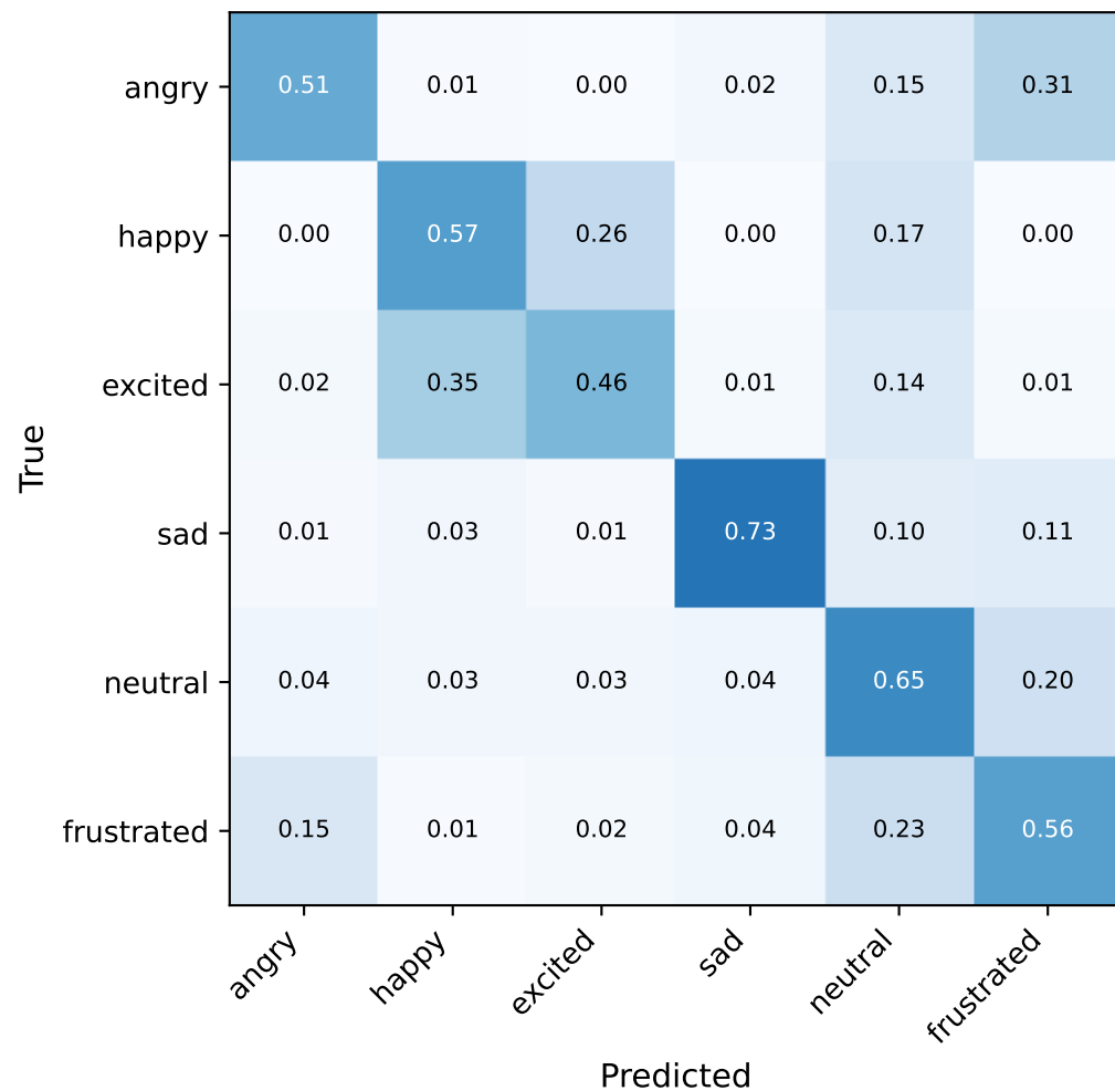
IEMOCAP (Full stack, seed 42)
