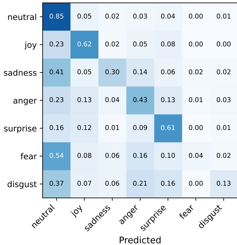
MELD (Full stack, seed 42)
