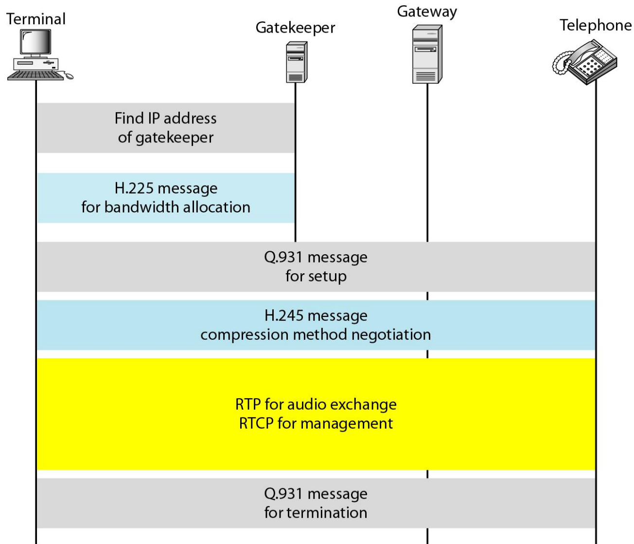
Figure 11.27 H.323 example
