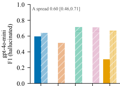
RAGTruth-Sum
