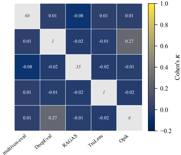
claude-haiku-4-5
