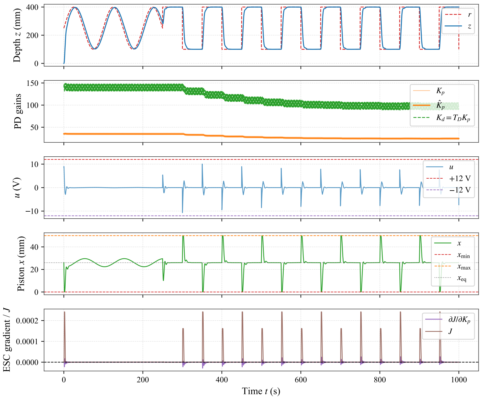
ESC-PD Depth Control: z(t) , Gains, u(t) , and x(t)
