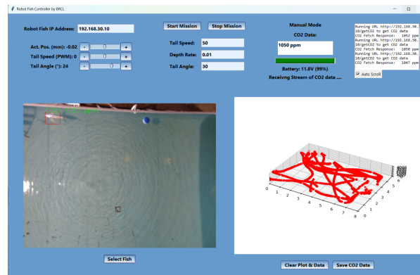
Fig. 5. Graphical User Interface (GUI) of the developed software for controlling the robotic fish and monitoring the \text{CO}_2 levels in water.
