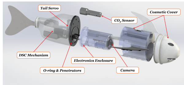
Fig. 2. Annotated CAD model of AquaNavigator robotic fish.
