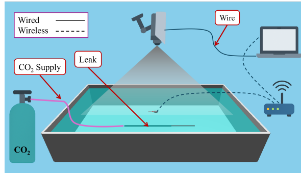
Fig. 7. Complete experimental setup for testing the robotic fish and monitoring the diffused CO 2 levels in water.
