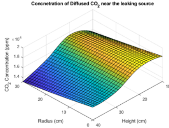
Fig. 4. Experimental results showing the diffusion of \text{CO}_2 in water at different depths and horizontal distances from the leak point.
