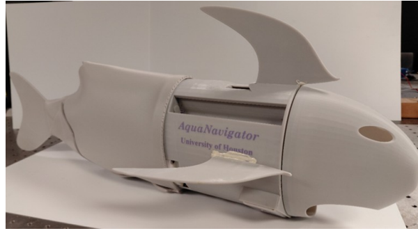
Fig. 1. Fabricated AquaNavigator robotic fish.
