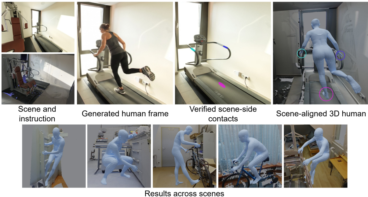
Figure 1: Overview and representative results. Given an interaction instruction, a calibrated scene view, and reconstructed scene geometry, our method generates a human interaction image, checks and refines body-part-specific scene contact regions, and fits a scene-aligned 3D human. The bottom row shows synthesized interactions across different scenes.
