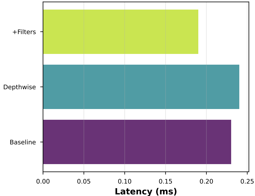
(b) Latency by Architecture
