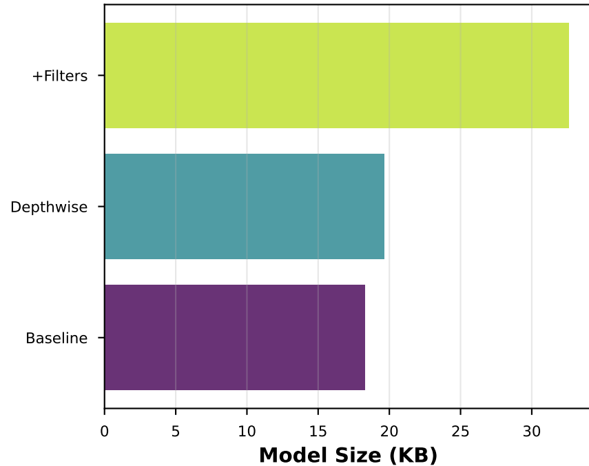
(c) Size by Architecture
