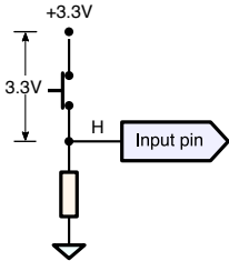
Switch pressed
