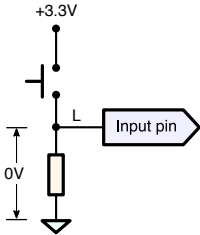
Switch released
