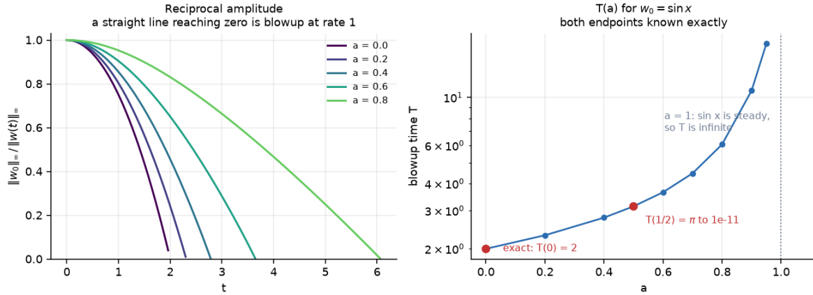
Figure 1: Left: reciprocal amplitude \|w_0\|_\infty / \|w(t)\|_\infty for several values of a . A straight line reaching zero is blowup with rate exponent one. Right: the blowup time T(a) from \omega_0 = \sin x , on a logarithmic scale. Both endpoints are known exactly, T(0) = 2 and T(1) = \infty , and the curve runs between them without any transition to global existence at intermediate a . The agreement of T(1/2) with \pi is marked but unexplained.
