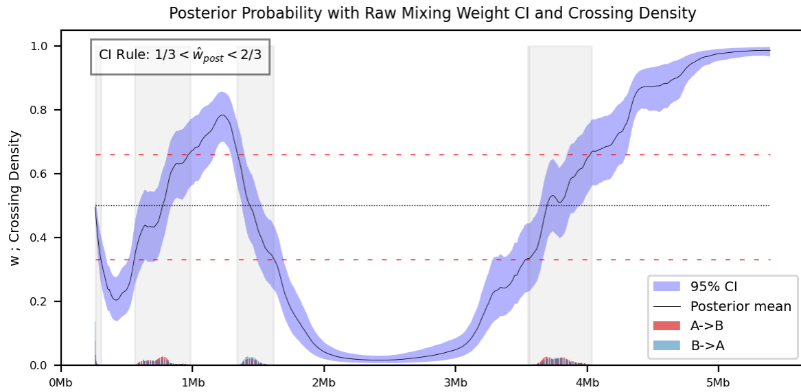
Figure 3.9: Posterior Probability with Raw Mixing Weight CI and Crossing Density. The CI rule used is 1/3 < \hat{w}_{post} < 2/3 , as shown. The grey band indicates the regions where the CI rule is not satisfied. The crossing density bars show the number of crossings of the posterior mean at 0.5, with red indicating crossings upwards and blue indicating crossings downwards.
