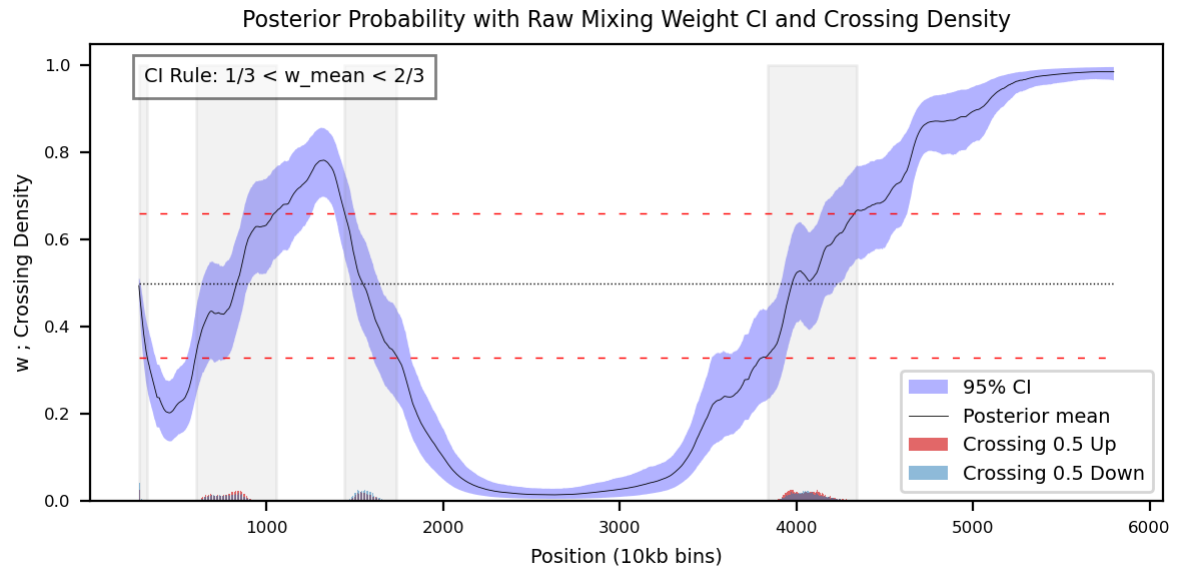
Figure 3.3: Posterior Probability with Raw Mixing Weight CI and Crossing Density. The CI rule used is 1/3 < w\_mean < 2/3 , as shown. The grey band indicates the regions where the CI rule is not satisfied. The crossing density bars show the number of crossings of the posterior mean at 0.5, with red indicating crossings upwards and blue indicating crossings downwards.
