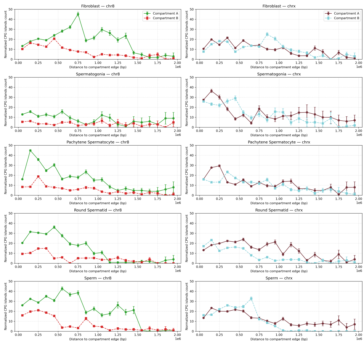
Figure 3.2: Figure: cpgislands
