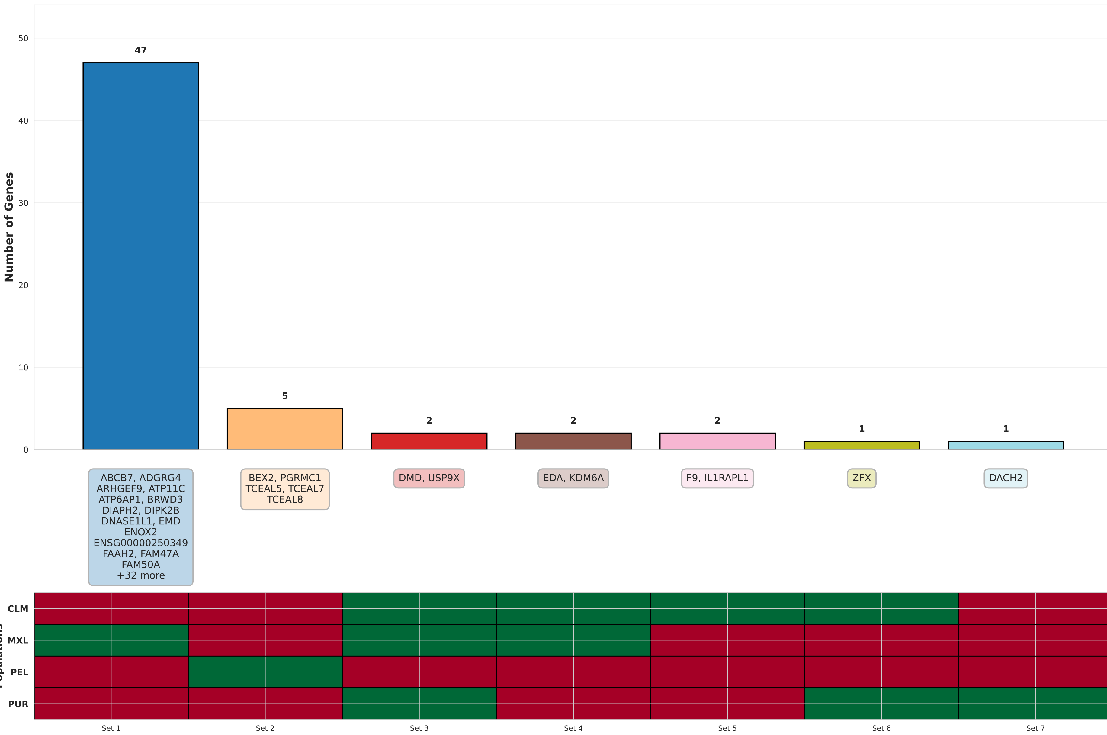
AMR: Protein-Coding Gene Overlaps Between Subpopulations
