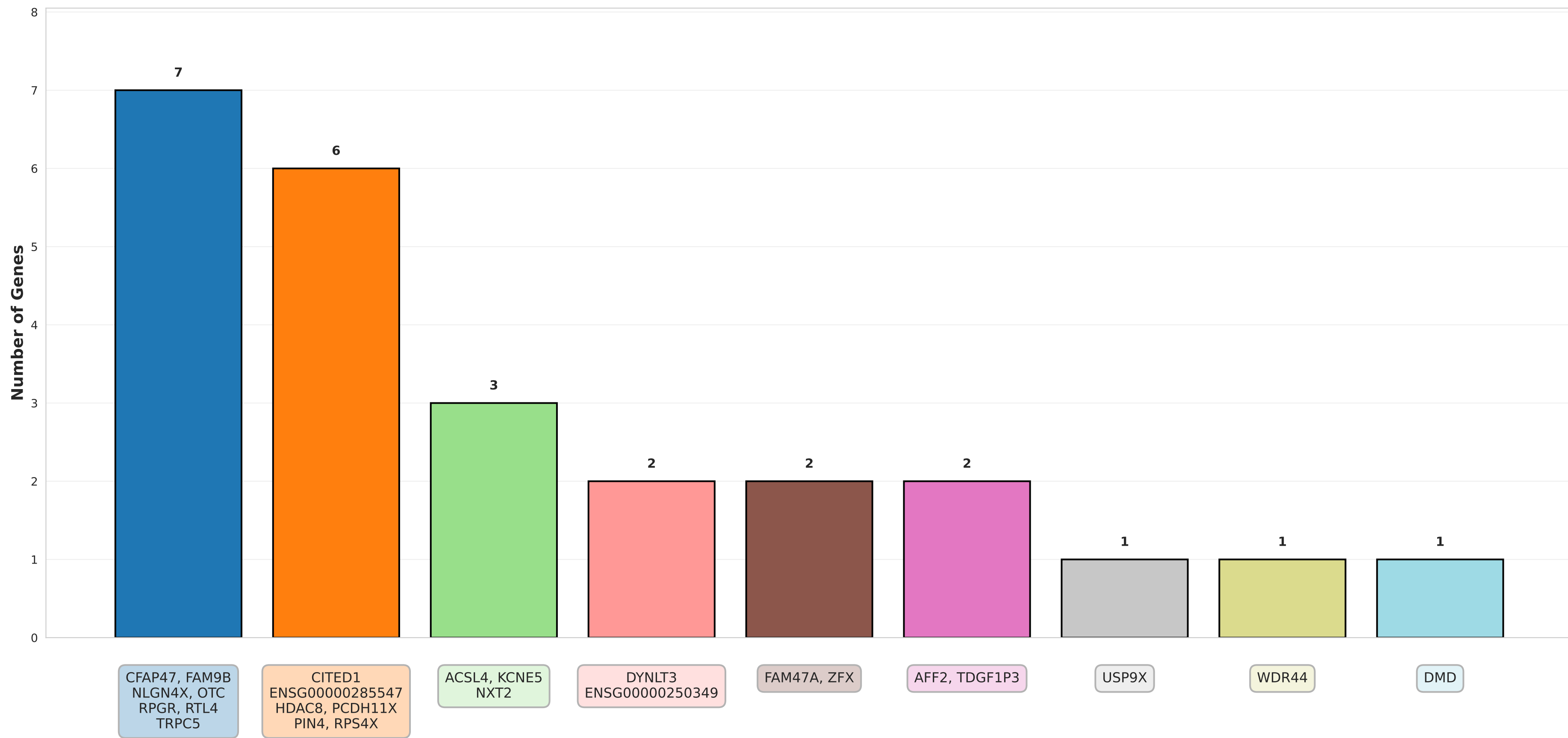
SAS: Protein-Coding Gene Overlaps Between Subpopulations
