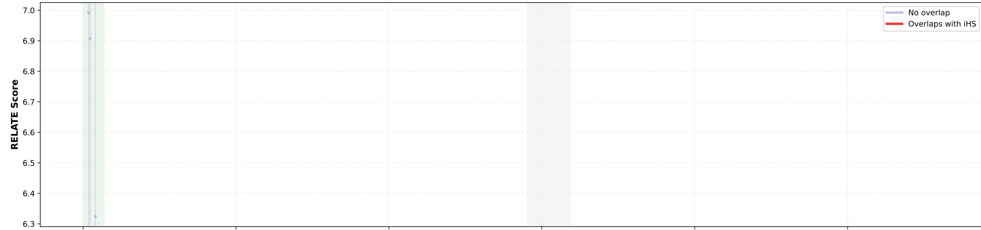
JPT: Overlapping Selection Regions (n=0)
