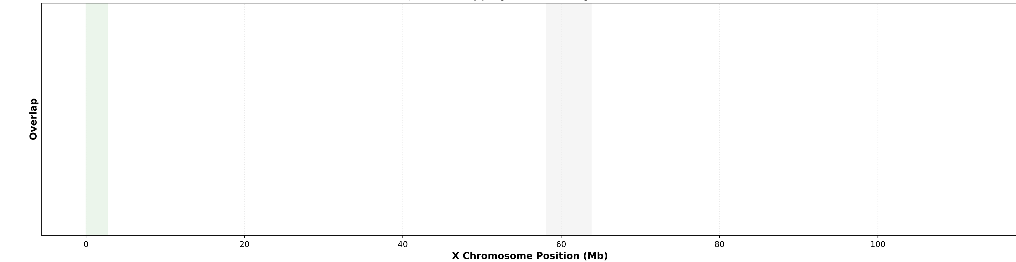
JPT: Overlapping Selection Regions (n=0)
