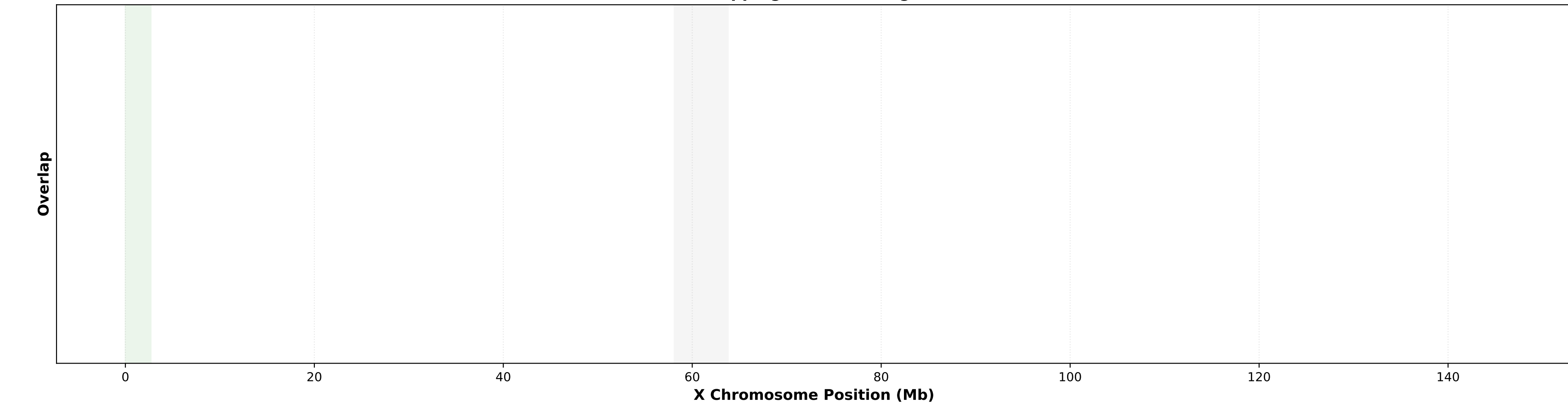
ESN: Overlapping Selection Regions (n=0)
