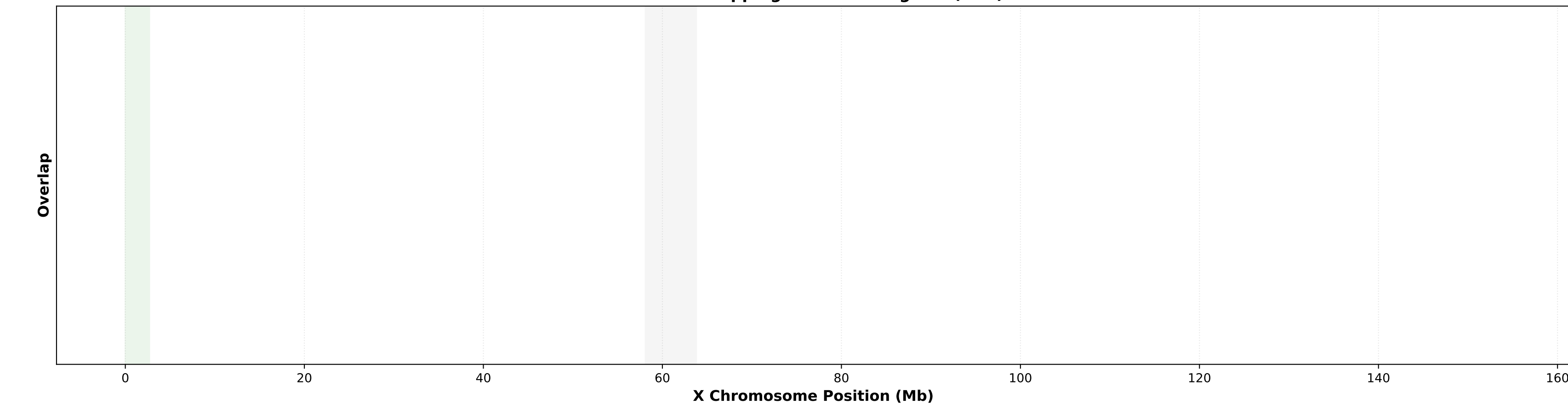
PUR: Overlapping Selection Regions (n=0)
