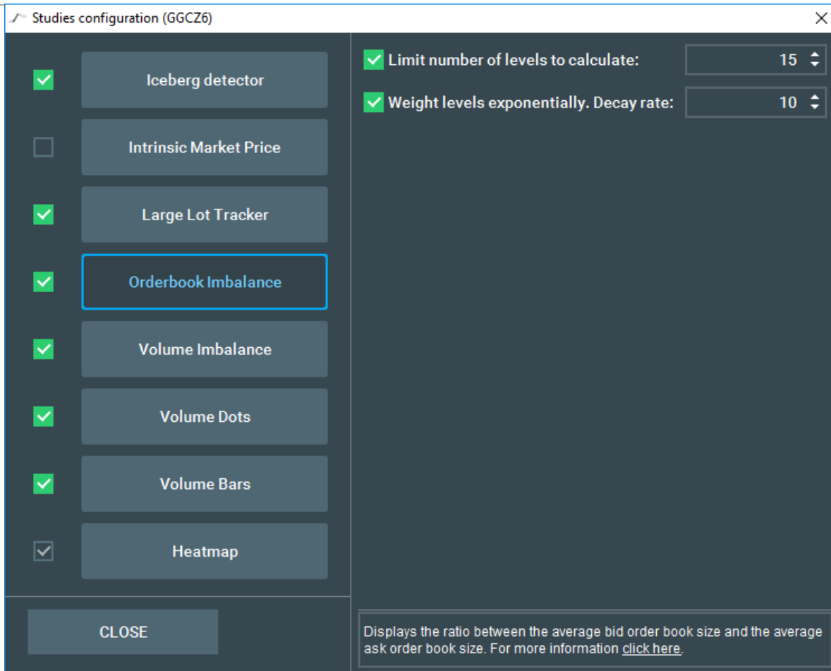
Imbalance Settings
