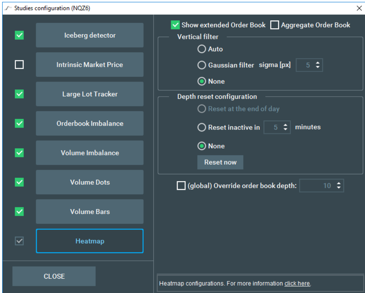
Heatmap Settings
