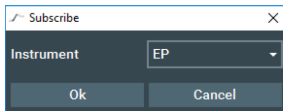
Instrument SubscriptionWindow
