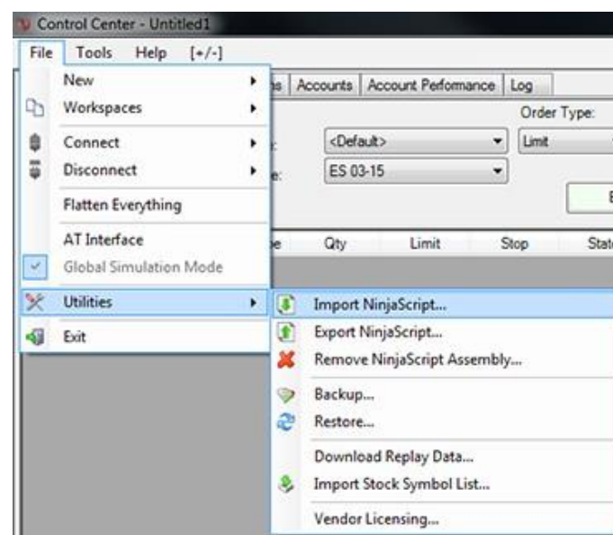
Importing NinjaScript
