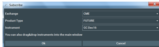
Instrument SubscriptionWindow
