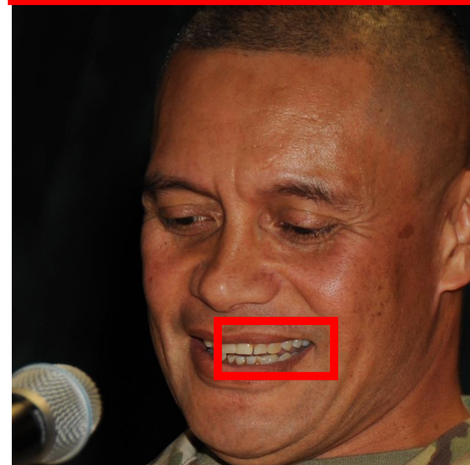
Ground Truth
