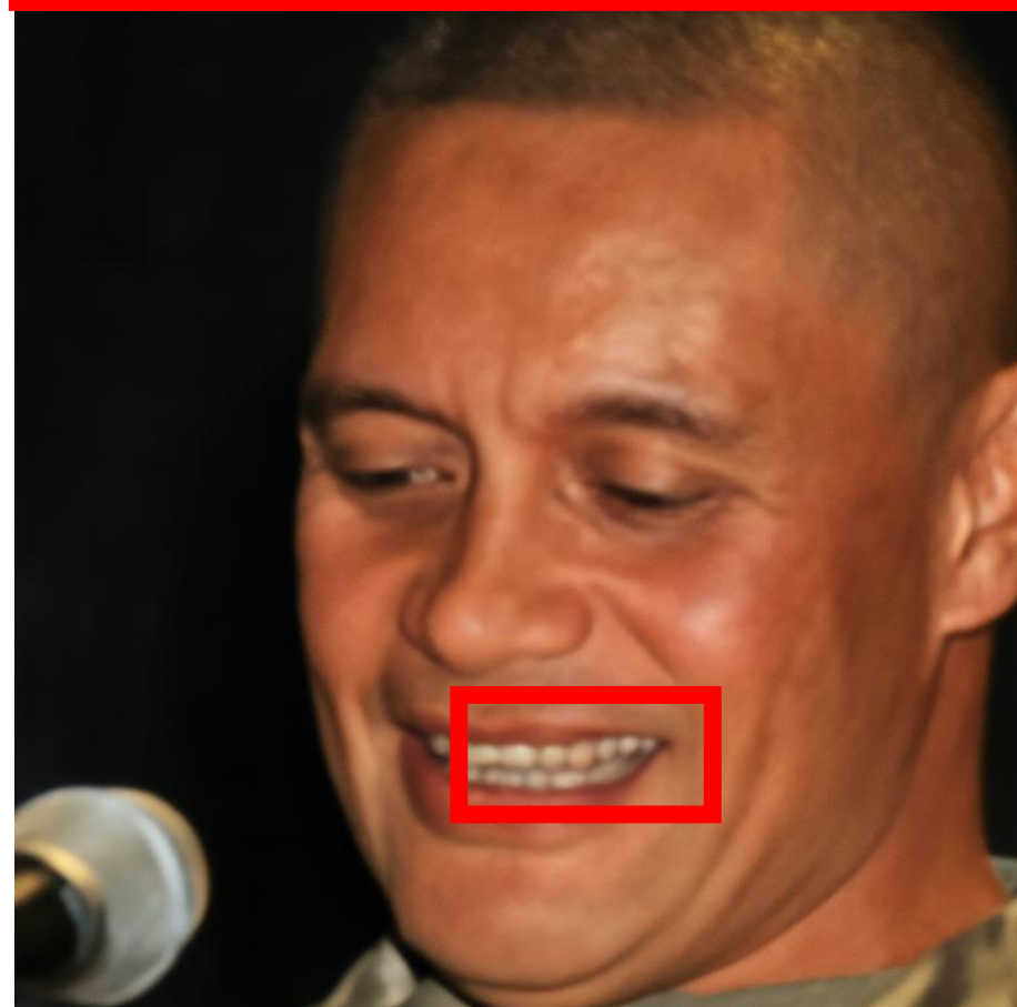
FlowDPS
