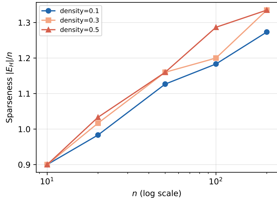
Greedy spanner, \alpha = 3 ( k = 2 )
