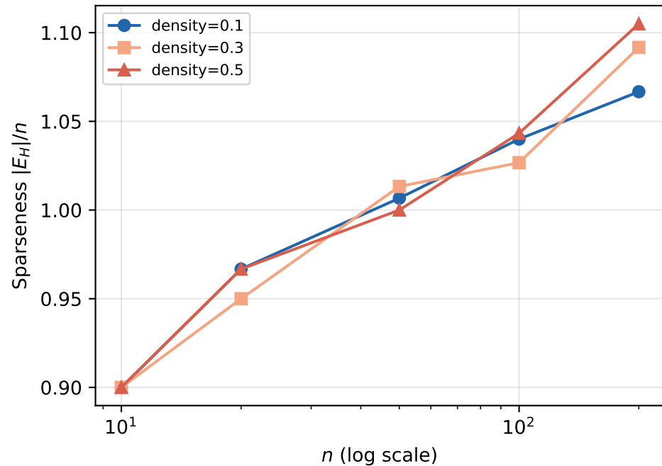
Greedy spanner, \alpha = 5 ( k = 3 )
