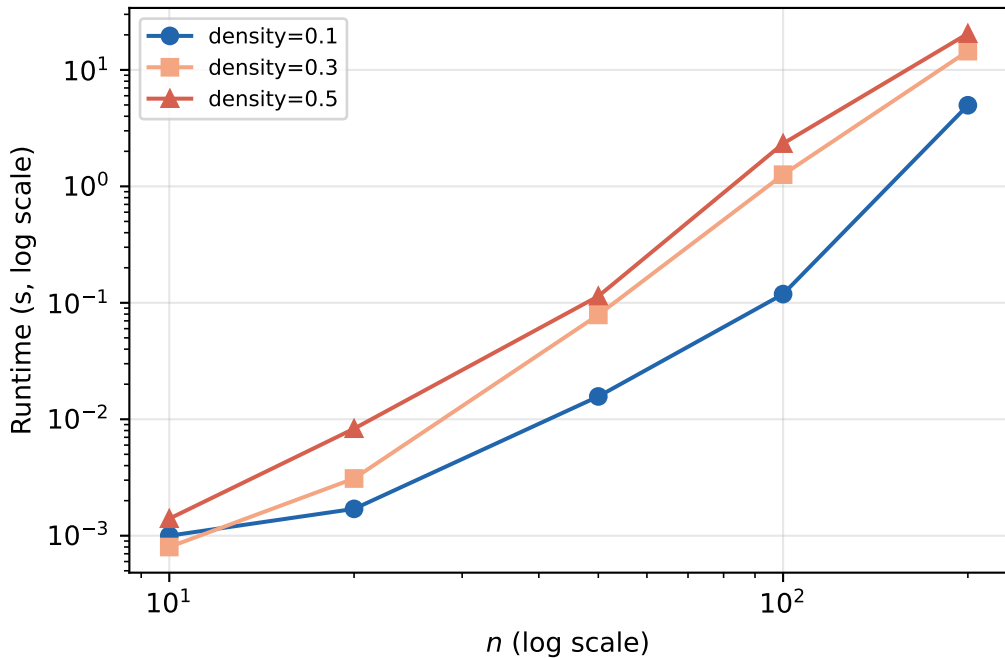
Greedy runtime ( \alpha = 3, k = 2 )
