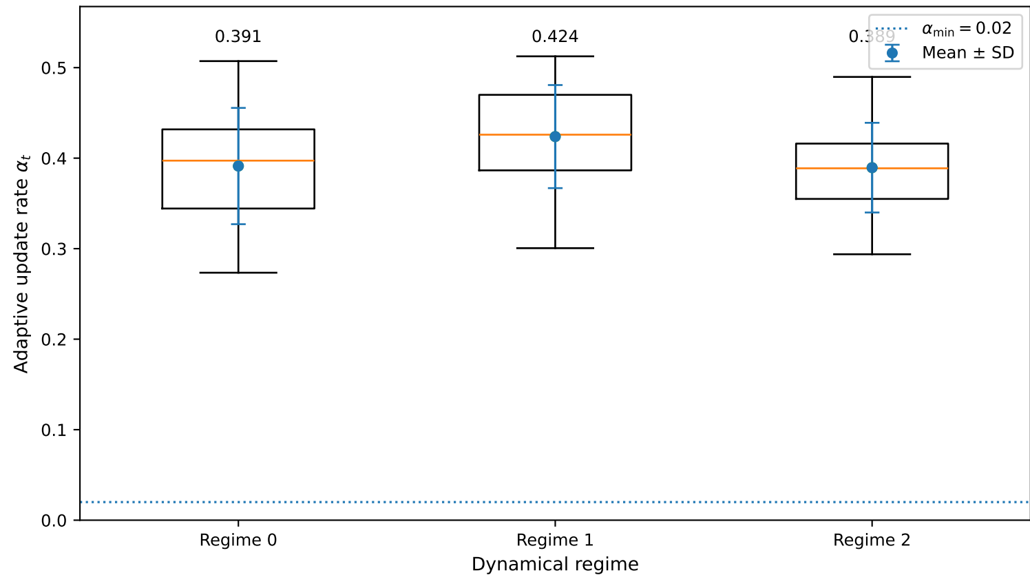
Adaptive Temporal Scaling Across Dynamical Regimes
