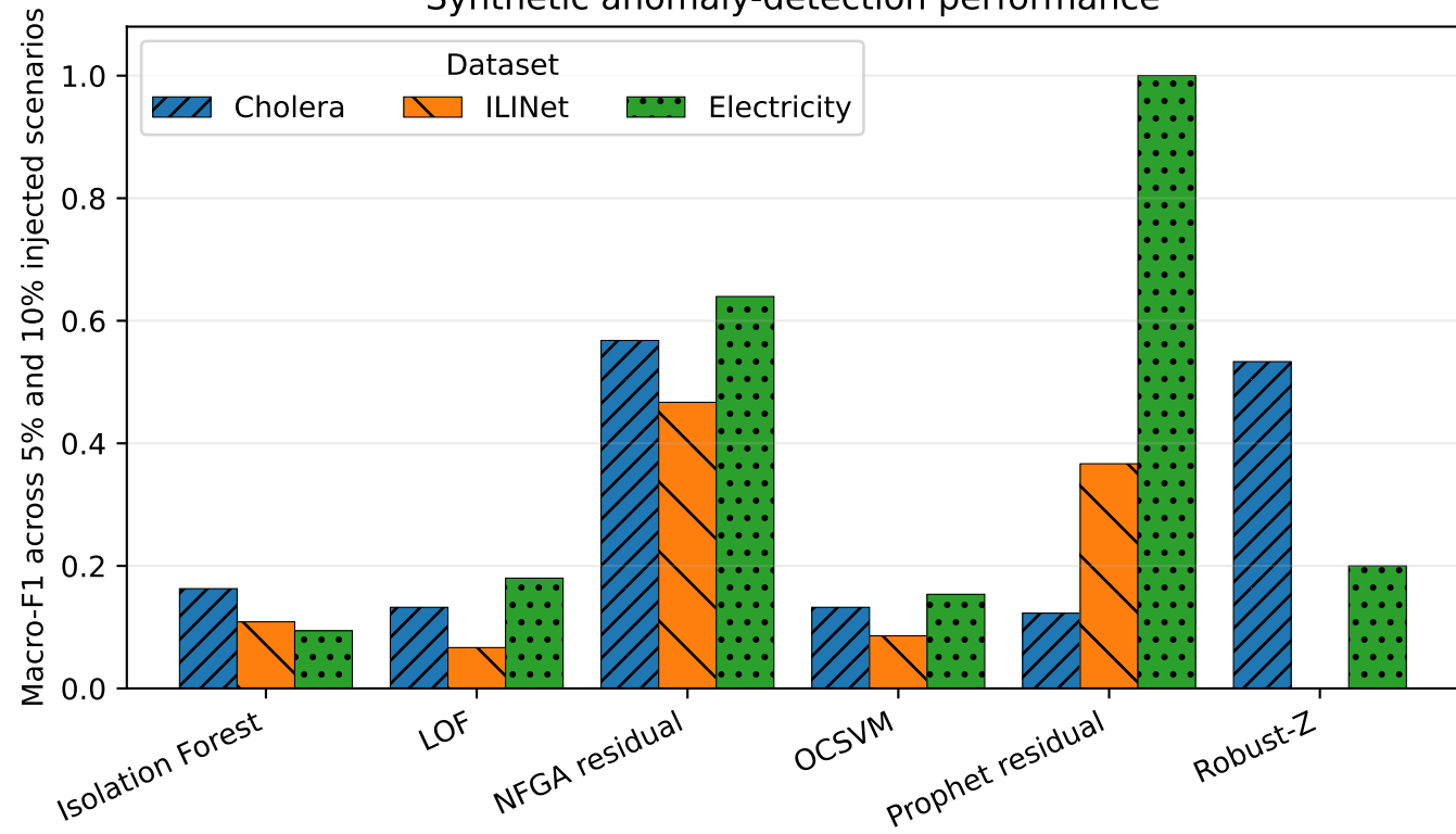
Synthetic anomaly-detection performance
