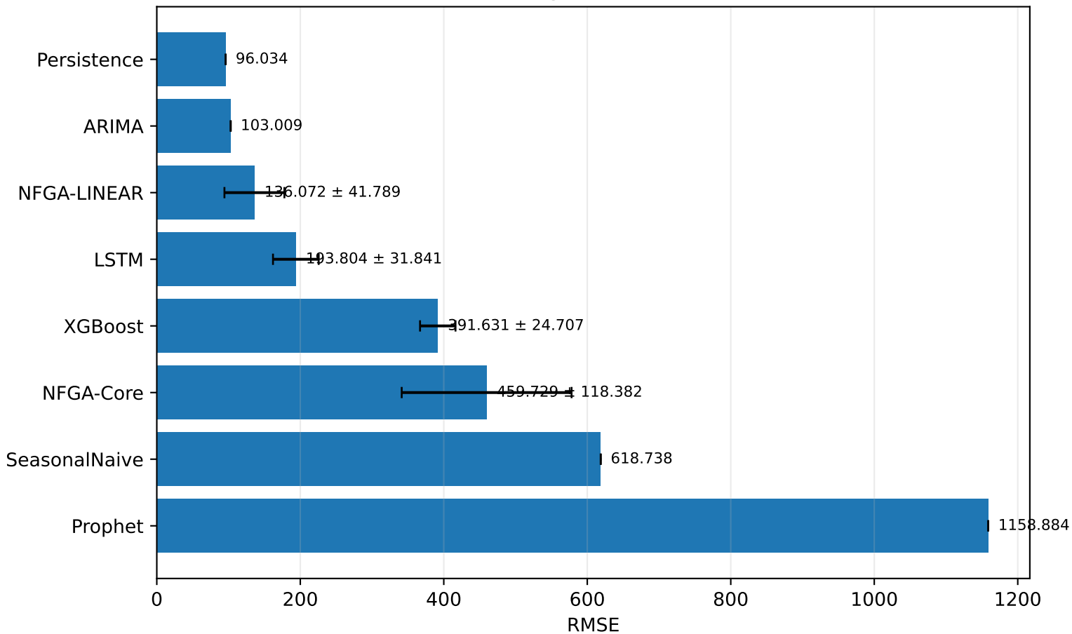
Forecasting RMSE — Cholera
