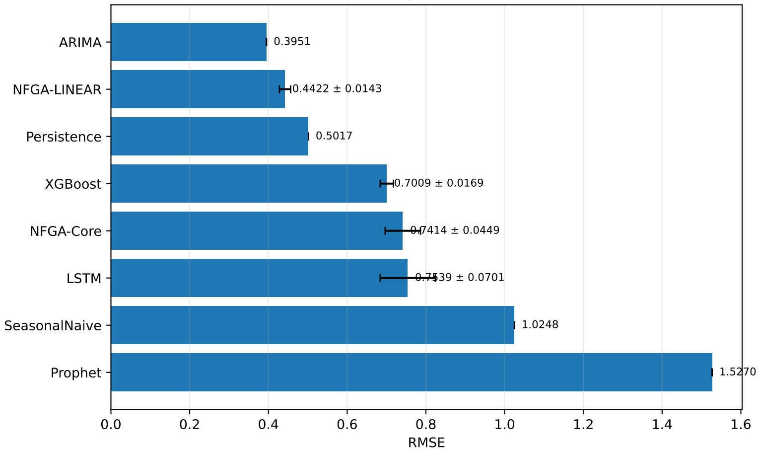
Forecasting RMSE — Ilinet
