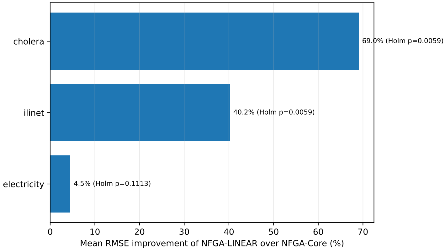
Matched ten-seed NFGA ablation
